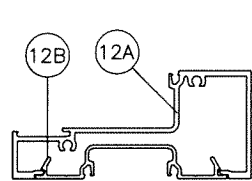
TRANSOM BAR HORIZONTAL MULLION WITHOUT REINF.
