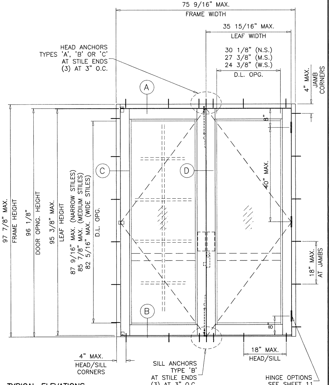
TYPICAL ELEVATIONS
