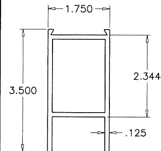
2 BOTTOM RAIL (NARROW STILE)
