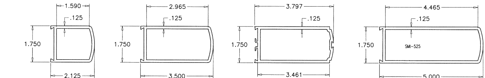
11 INACTIVE LOCK STILE (NARROW STILE) 11A INACTIVE LOCK STILE (MEDIUM STILE) 11.1A ALT. INACTIVE LOCK STILE (MEDIUM STILE) 11B INACTIVE LOCK STILE (WIDE STILE)
