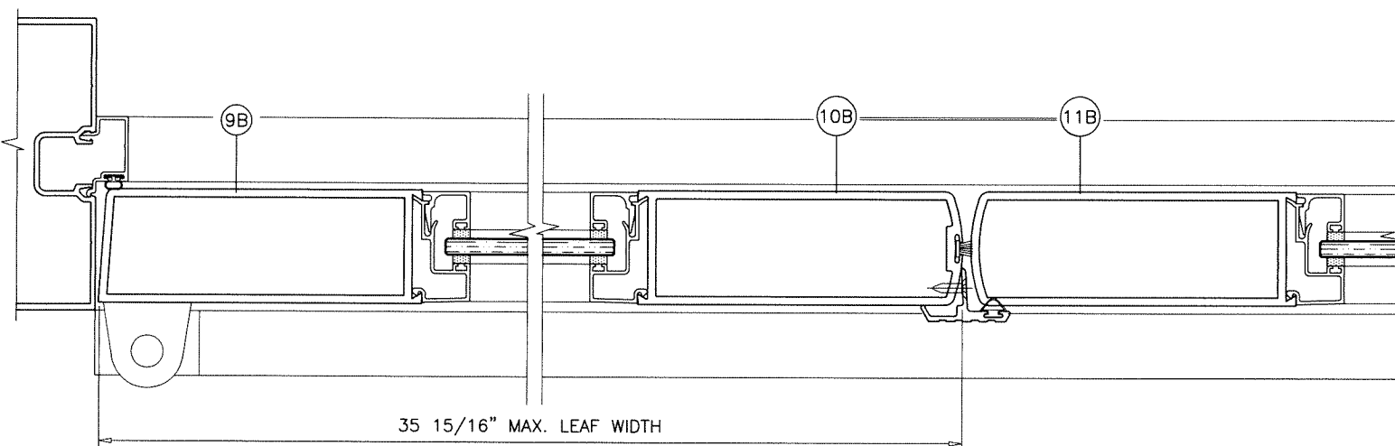
WIDE STILE DOOR DOUBLE DOOR (XX)
