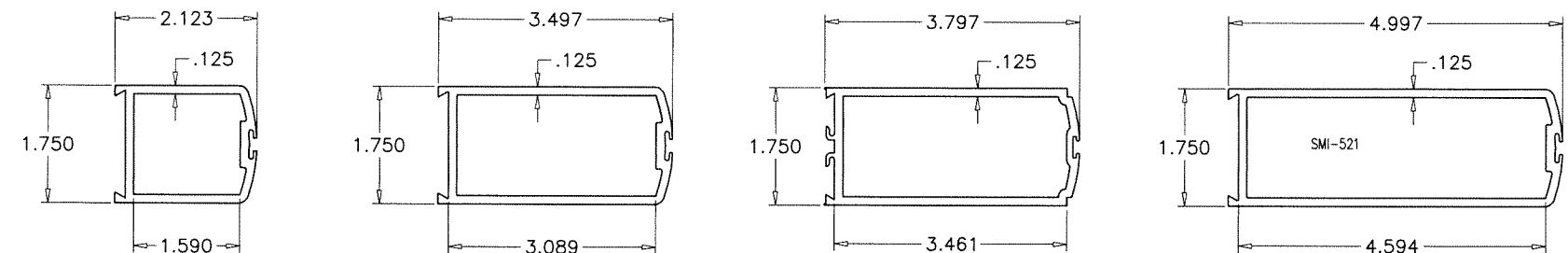
10 ACTIVE LOCK STILE (NARROW STILE) 10A ACTIVE LOCK STILE (MEDIUM STILE) 10.1A ALT. ACTIVE LOCK STILE (MEDIUM STILE) 10B ACTIVE LOCK STILE (WIDE STILE)
