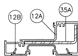
TRANSOM BAR HORIZONTAL MULLION WITH REINF.
